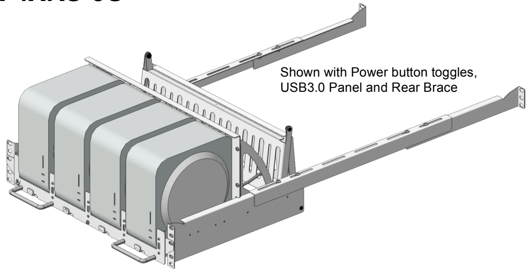
Shown with Power button toggles, USB3.0 Panel and Air Baffle
